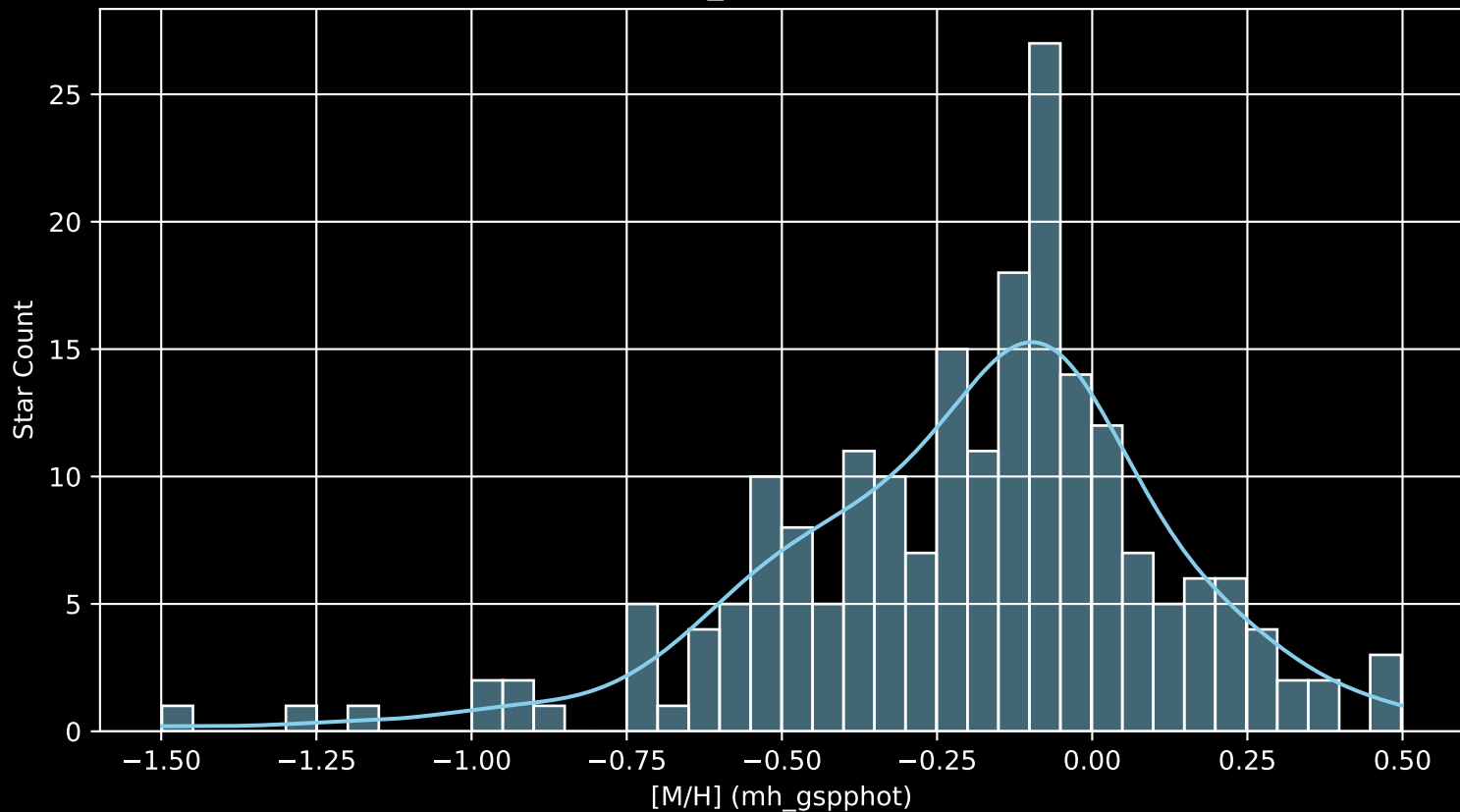
APOGEE DR17 Field: [270-40-O_TESS] [M/H] (mh_gspphot) (n= 206)
