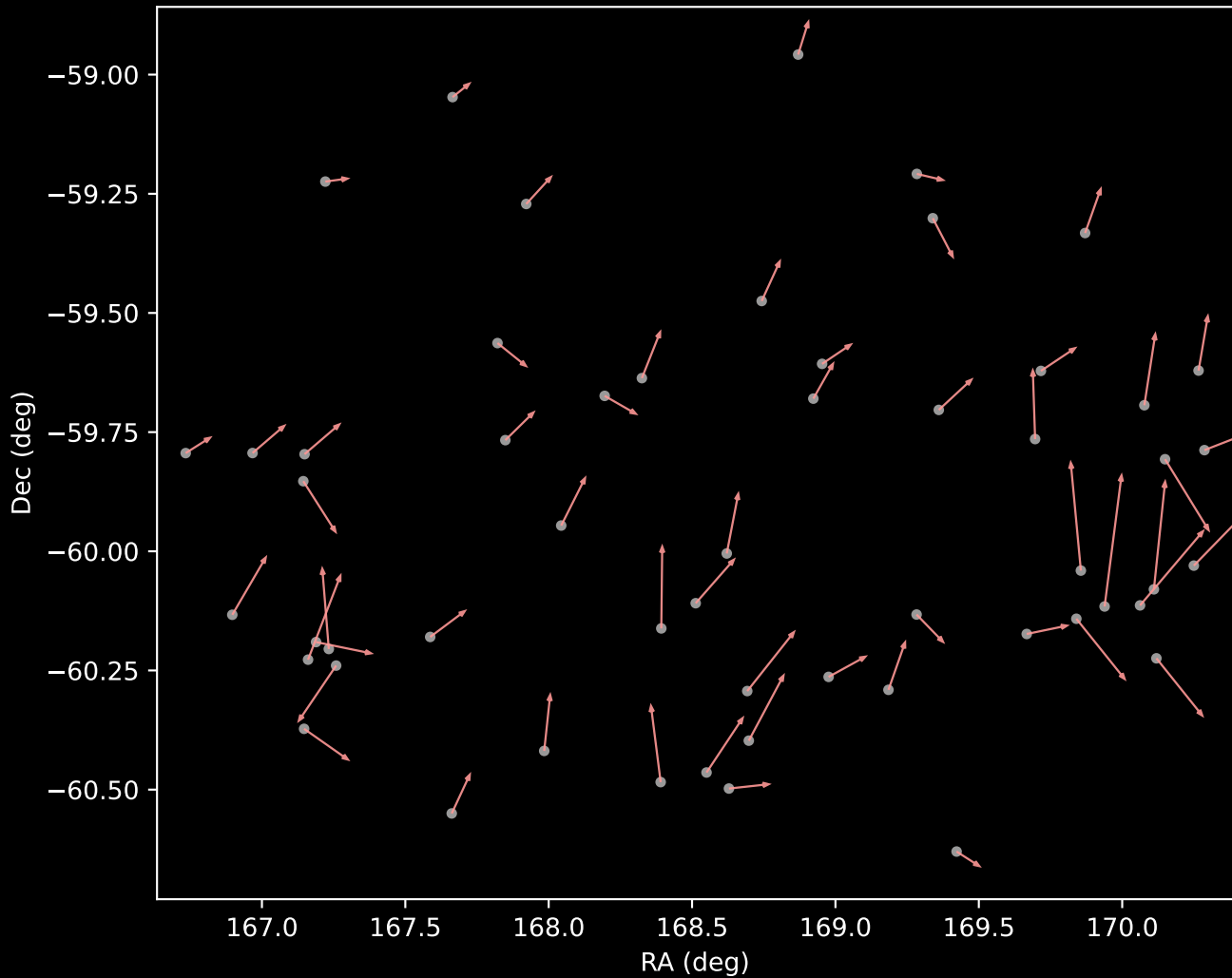
APOGEE DR17 Cluster 7 Proper Motion Vectors (n=55)
