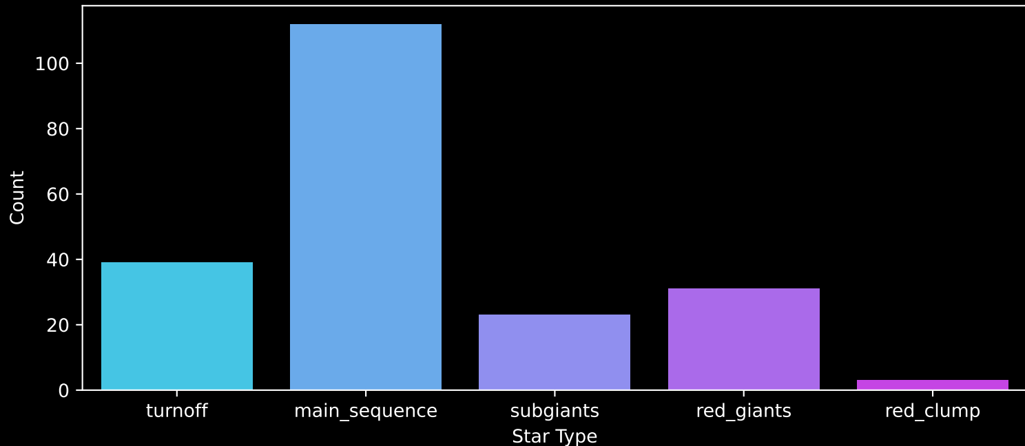
APOGEE DR17 Field: [270-40-O_TESS] Count plot of Star Type
