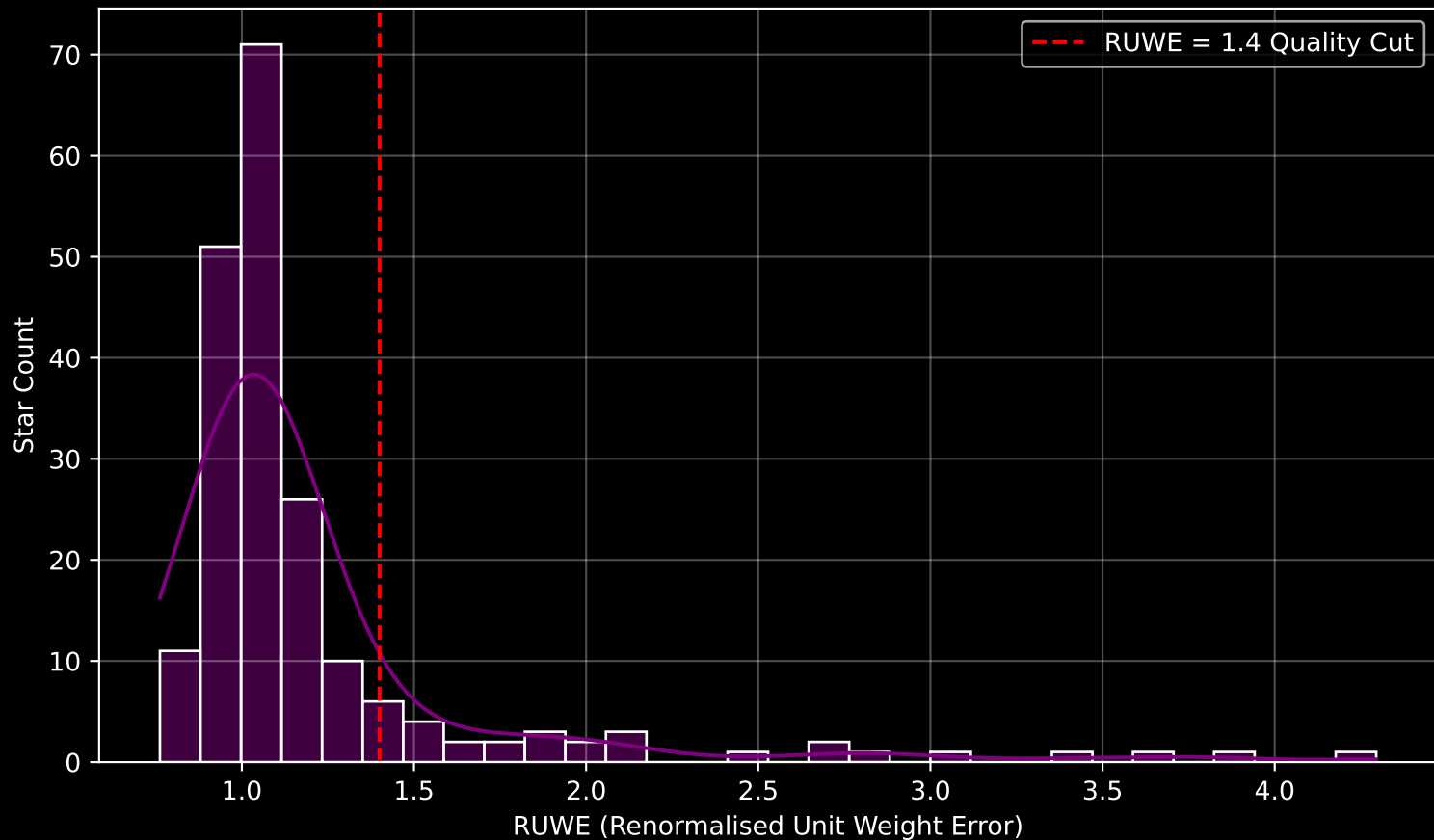
GAPOGEE DR17 Field [270-40-O_TESS] RUWE Distribution (n= 200)
