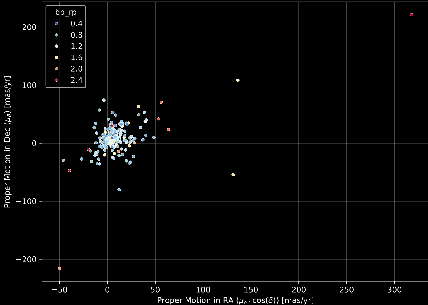
APOGEE DR17 Field: [270-40-O_TESS] Proper Motion Diagram (n= 208)
