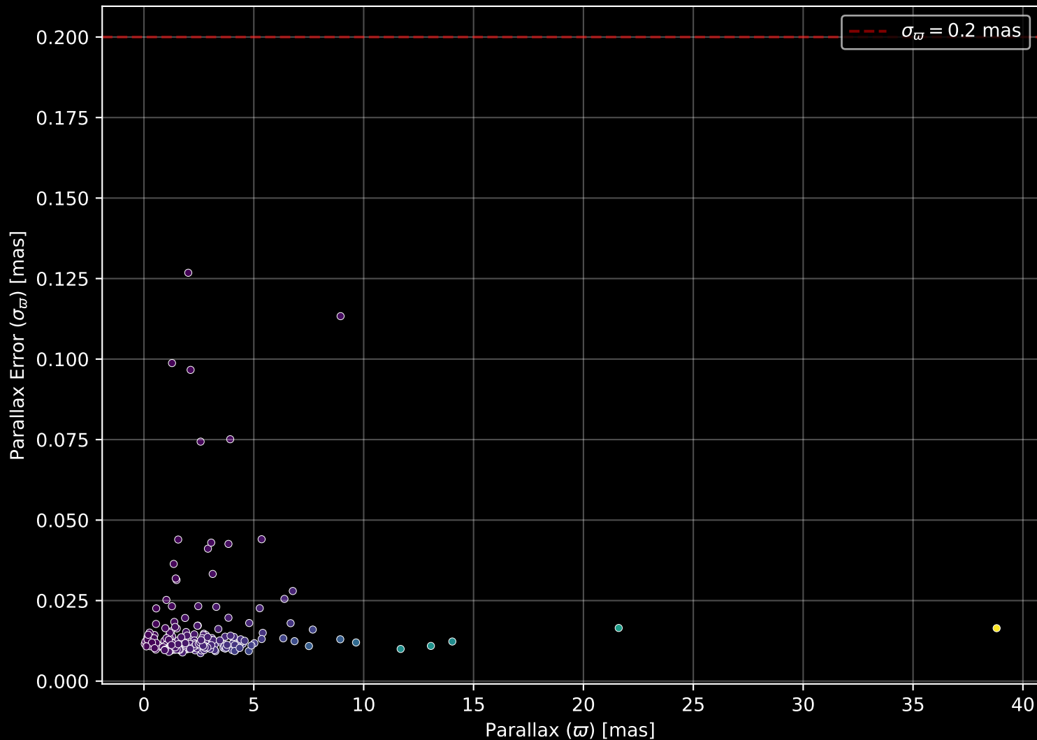
APOGEE DR17 Field: [270-40-O_TESS] Parallax Quality (n= 208)
